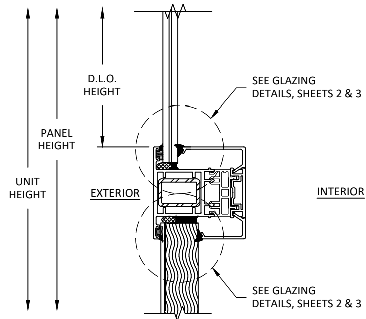
Q 14 VERTICAL SECTION ALS-C MIDRAIL - GLASS OVER INFILL PANEL REINFORCED
