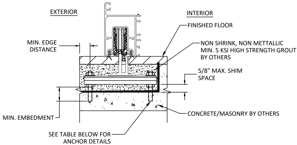
N 21 VERTICAL SECTION 1-TRACK SILL - THROUGH FRAME
