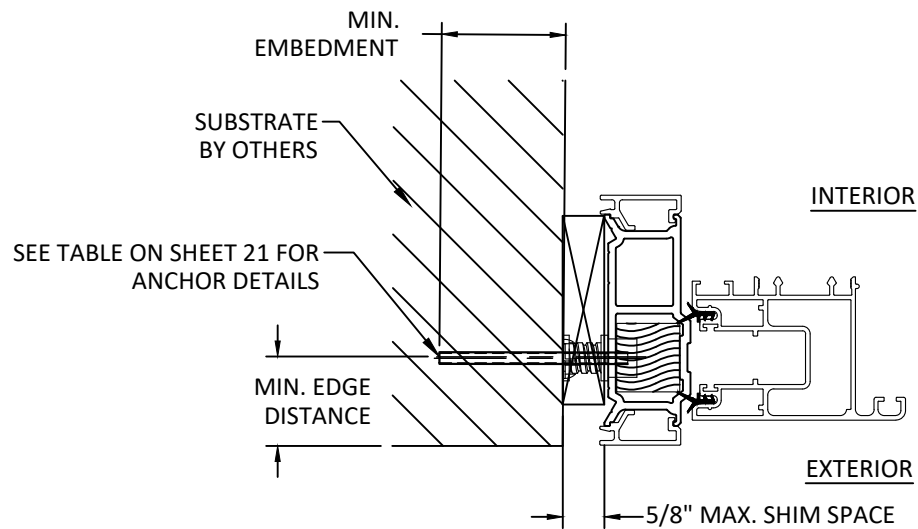
P 22 VERTICAL SECTION 1 TRACK JAMB - THROUGH FRAME
