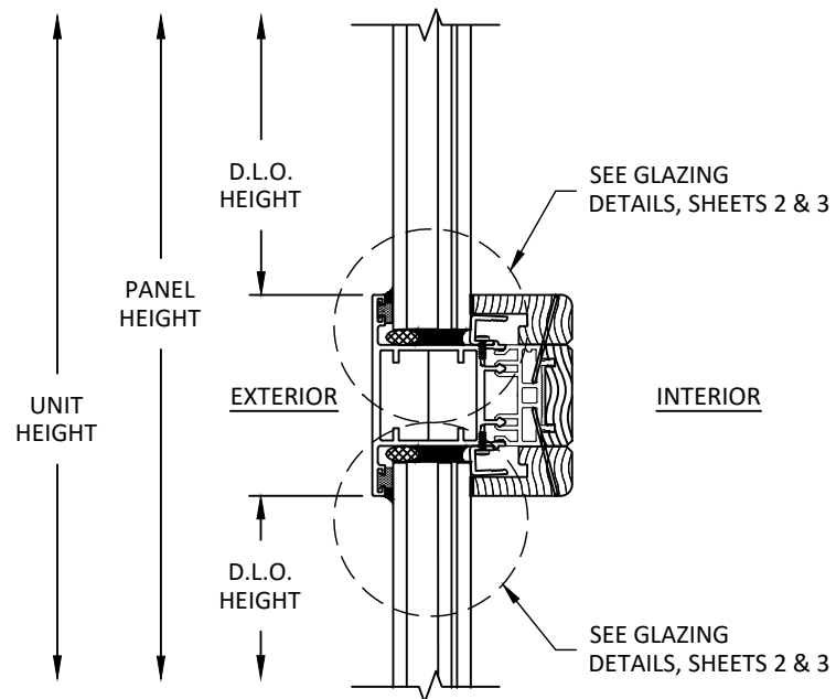
G 12 VERTICAL SECTION AWLS-C MIDRAIL - GLASS OVER GLASS NON - REINFORCED
