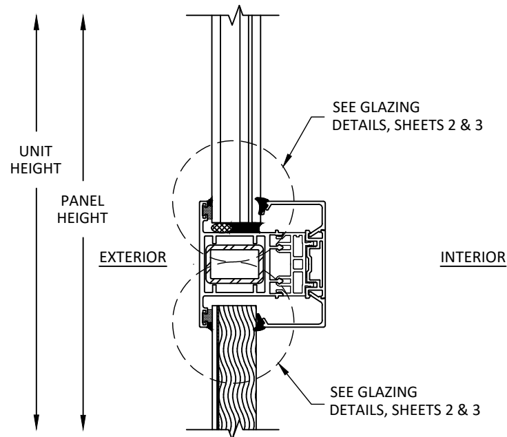
R 14 VERTICAL SECTION ALS-C MIDRAIL - INFILL OVER INFILL REINFORCED
