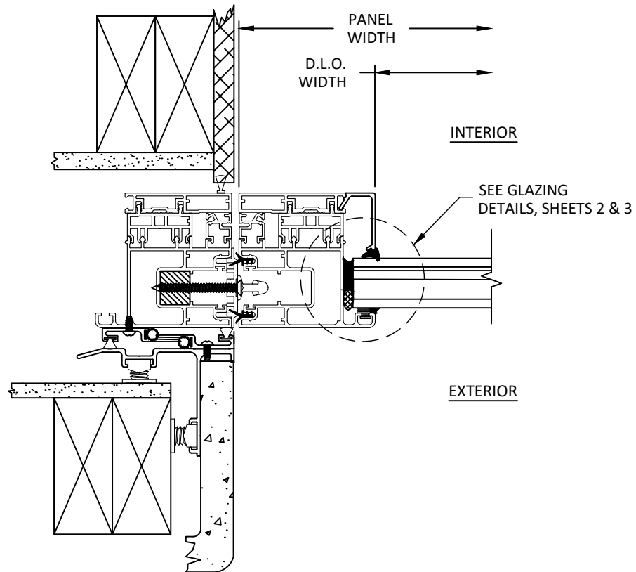
L 20 HORIZONTAL SECTION ALS-C 1-TRACK WALL JAMB
