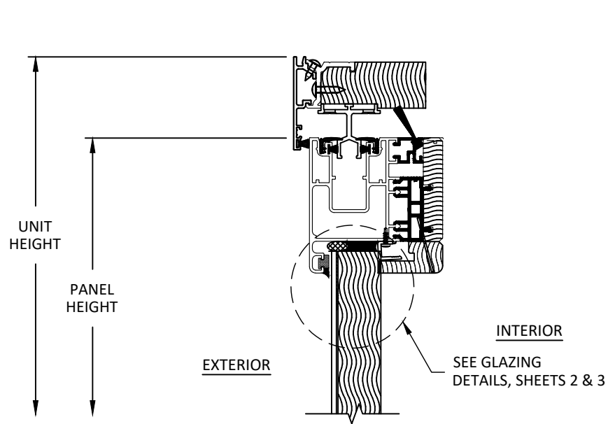
E 12 VERTICAL SECTION AWLS-C HEAD 1 TRACK
