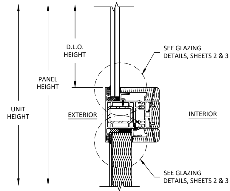
I 12 VERTICAL SECTION AWLS-C MIDRAIL - GLASS OVER INFILL PANEL REINFORCED
