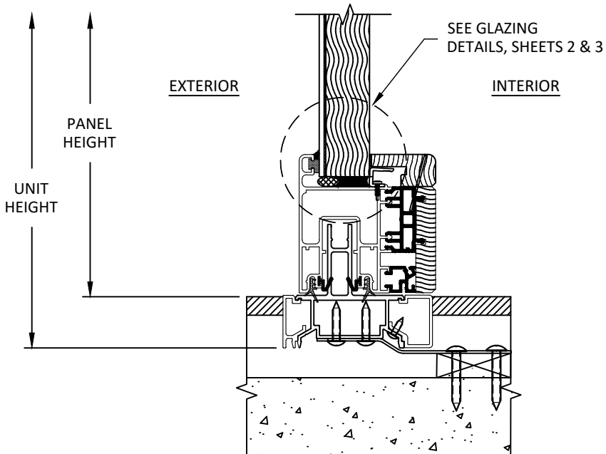
CC 16 VERTICAL SECTION AWLS-C SILL H TRACK
