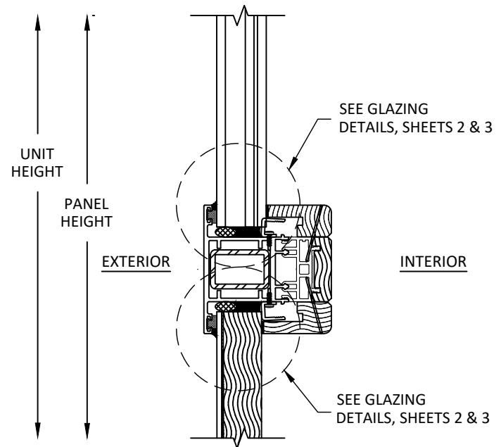
H 12 VERTICAL SECTION AWLS-C MIDRAIL - INFILL OVER INFILL REINFORCED
