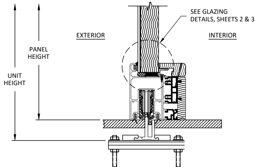
F 12 VERTICAL SECTION AWLS-C SILL 1 TRACK
