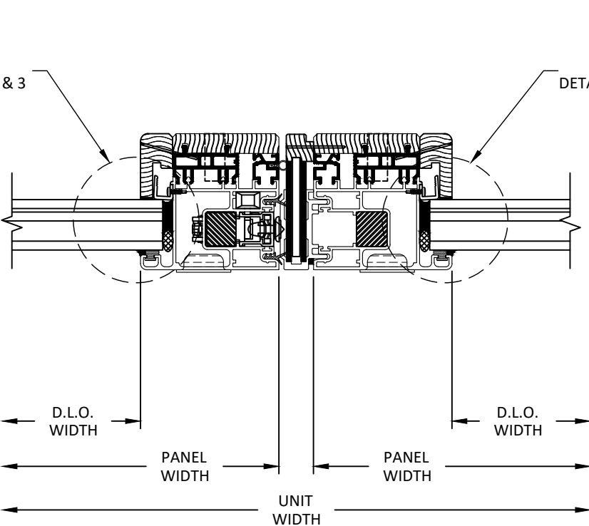
T 15 HORIZONTAL SECTION AWLS-C MEETING STILE
