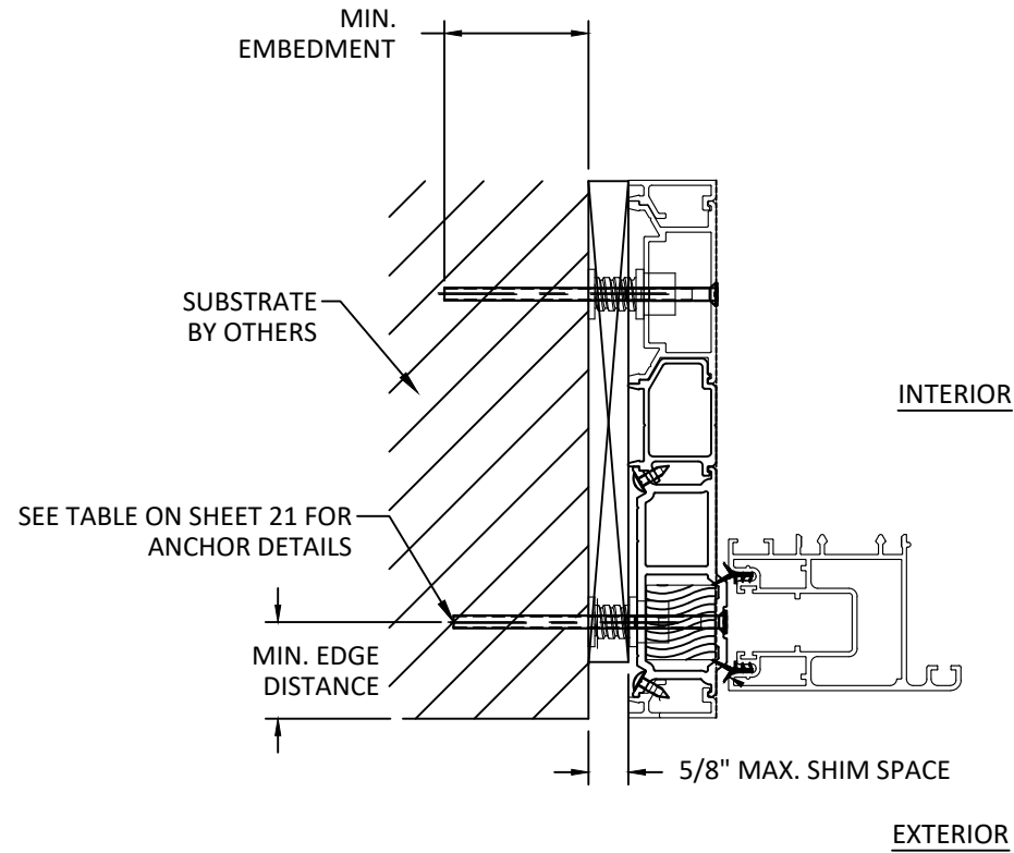
Q 22 VERTICAL SECTION 2 TRACK JAMB - THROUGH FRAME
