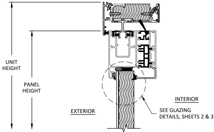
N 14 VERTICAL SECTION ALS-C HEAD 1 TRACK
