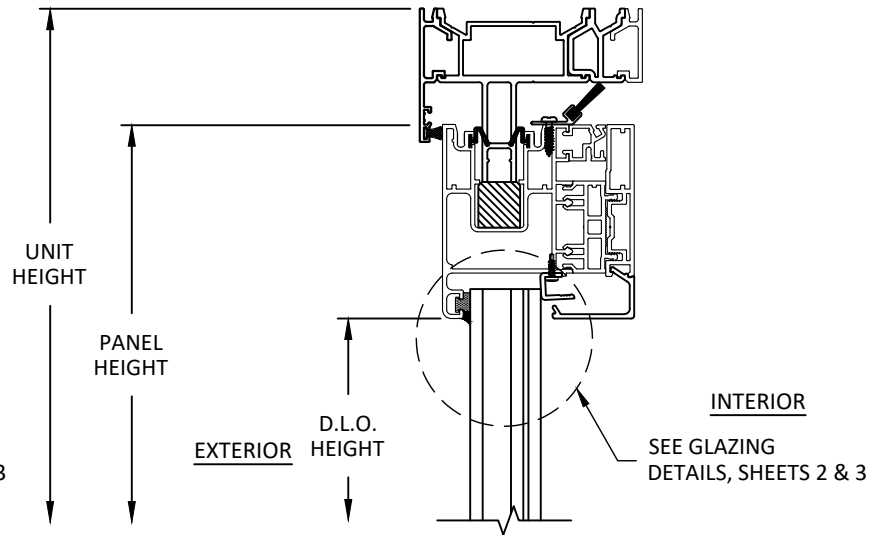
N 14 VERTICAL SECTION ALS-C HEAD H TRACK
