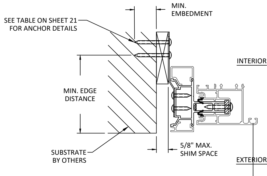
R 22 HORIZONTAL SECTION 1 TRACK JAMB - H TRACK
