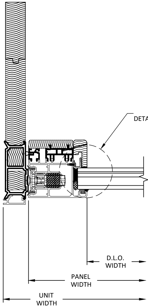
S 15 HORIZONTAL SECTION AWLS-C JAMB 3 TRACK
