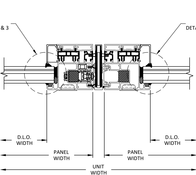
F 18 HORIZONTAL SECTION ALS-C MEETING STILE
