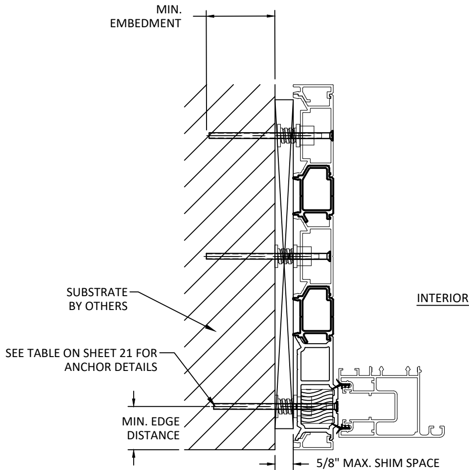
O 22 VERTICAL SECTION 3 TRACK JAMB - THROUGH FRAME
