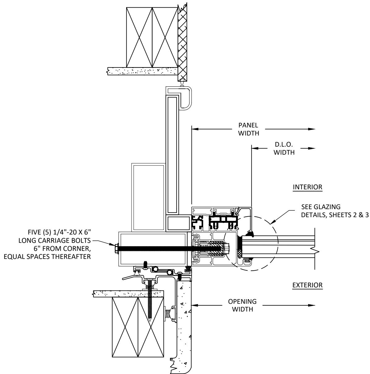
J 20 HORIZONTAL SECTION ALS-C 3-TRACK POCKET JAMB
