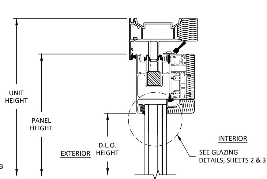
AA 12 VERTICAL SECTION AWLS-C HEAD H TRACK
