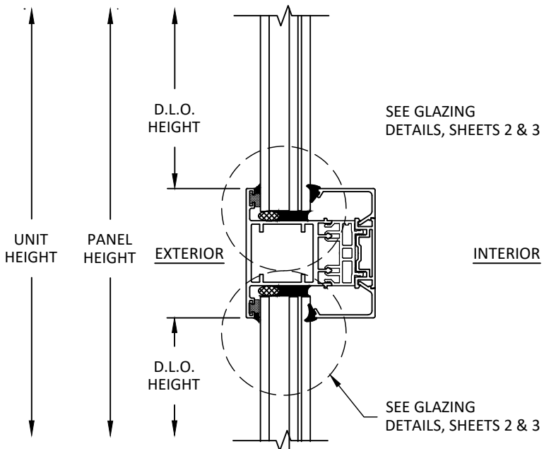
P 14 VERTICAL SECTION ALS-C MIDRAIL - GLASS OVER GLASS NON - REINFORCED
