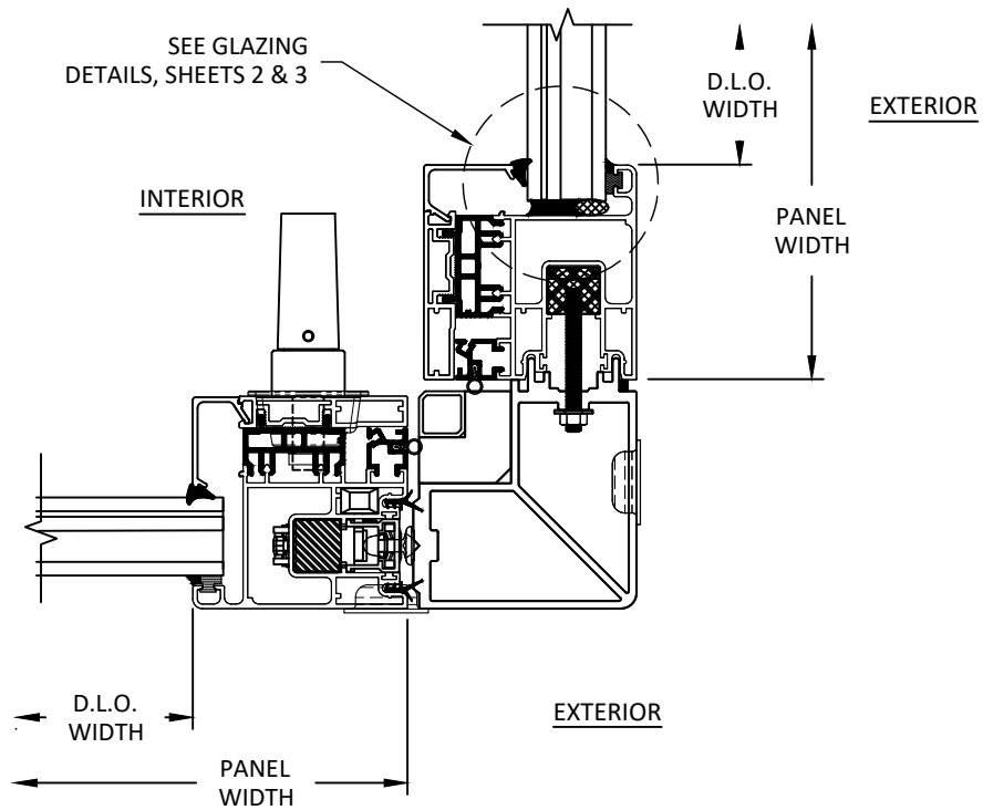
K 20 HORIZONTAL SECTION ALS-C 90° CORNER POST
