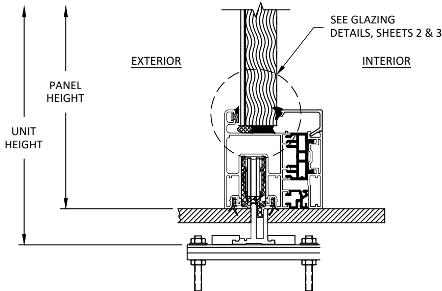
O 14 VERTICAL SECTION ALS-C SILL 1 TRACK
