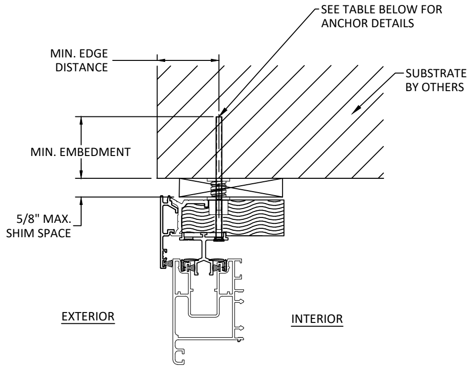
M 21 VERTICAL SECTION 1-TRACK HEAD - THROUGH FRAME
