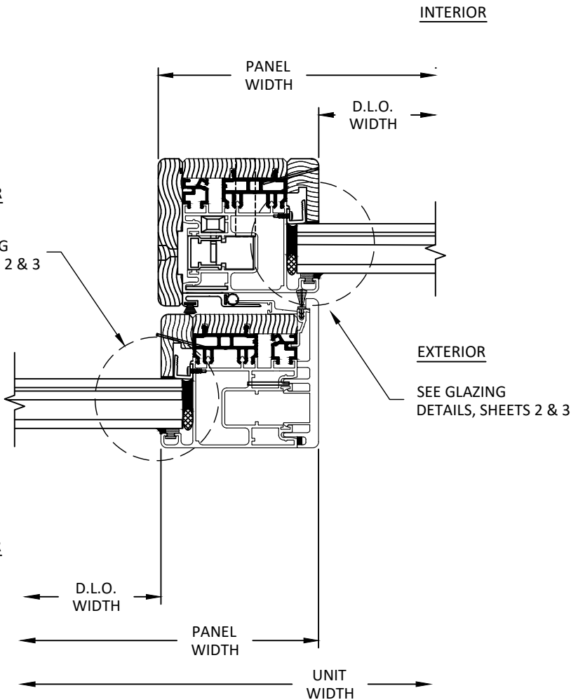
U 15 HORIZONTAL SECTION AWLS-C INTERLOCK
